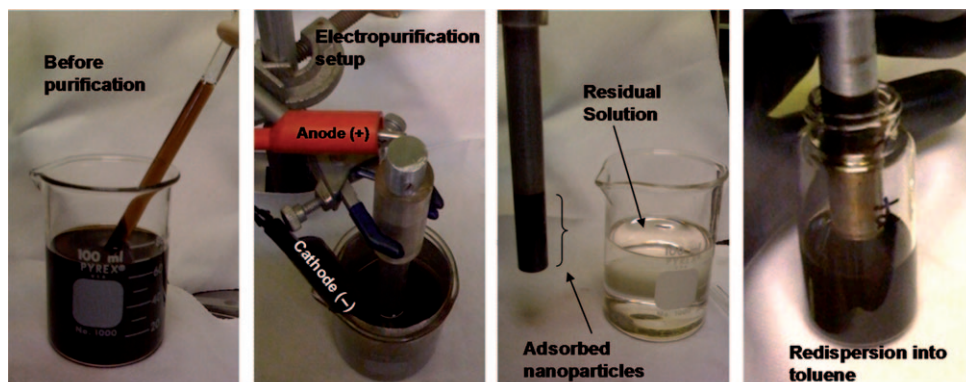
Figure 1. Electropurification process showing, from left to right, an as-synthesized nanoparticle solution (CdTe) before, during, and after reversible deposition on the electrode. The final frame shows the redispersion of the nanoparticles into clean solvent, contrasting the bottom of the electrode, which has been exposed to toluene and is clean, with the top of the electrode, which still contains adsorbed nanoparticles.
